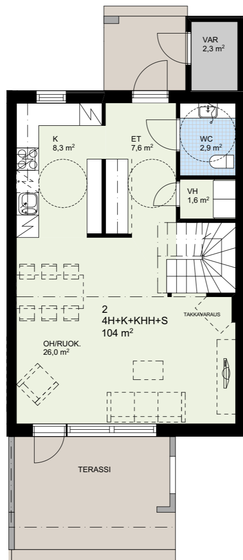
HSTO 2 1.krs 1:100
