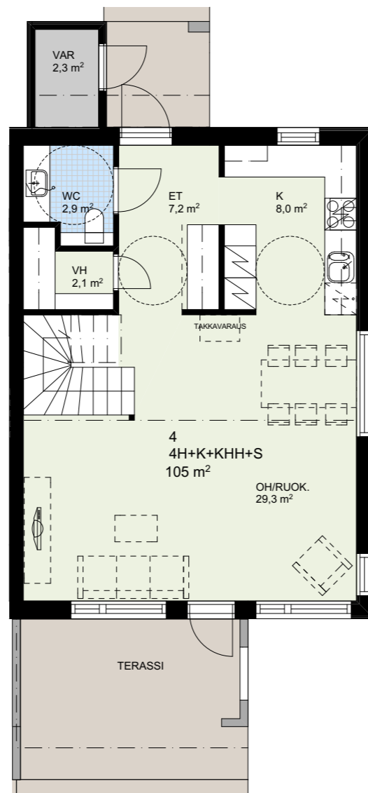
HSTO 4 1.krs 1:100
